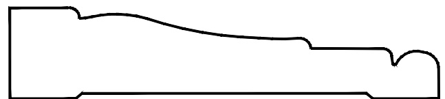
445 Casing 11/16 \times 3-1/4
