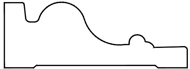
222 Casing 1-1/16 \times 3-1/4
