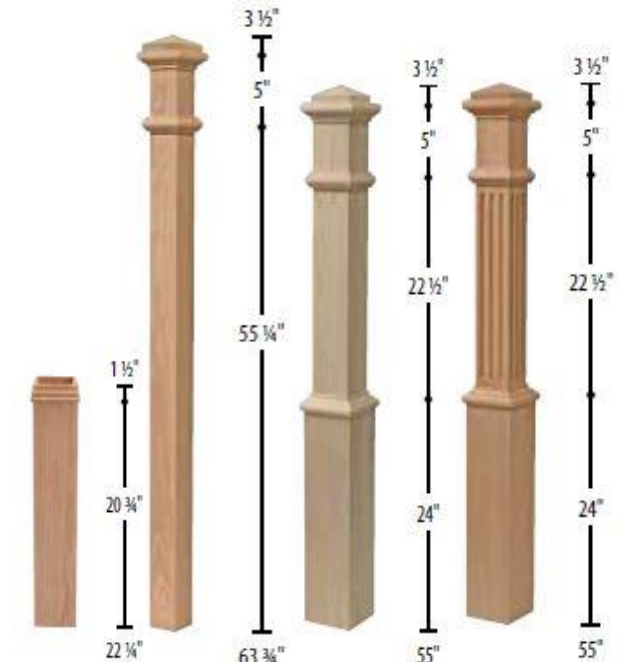
SW-4075SL 22 1/4" Starting Newel SW-4075 20 3/4" Starting Newel SW-4091 63 3/4" Starting Newel SW-4091F 5-1/2" & SW-4091XLF 6-1/4" Starting Newel SW-4091F 22 1/2" Landing Newel SW-4091XLF 22 1/2" Landing Newel
