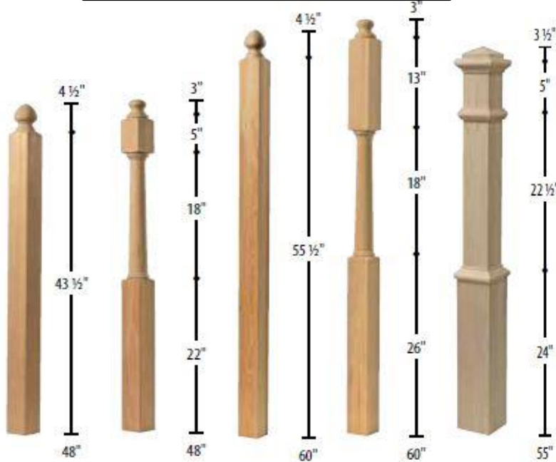
SW-H4004 HEMLOCK 3-1/4" STARTING NEWEL SW-H4040 HEMLOCK 3-1/4" STARTING NEWEL SW-H4005 HEMLOCK 3-1/4" LANDING NEWEL SW-H4046 HEMLOCK 3-1/4" LANDING NEWEL SW-4091 POPLAR BOX NEWEL
