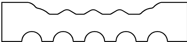
Classic Trim 11/16 \times 3-1/4
