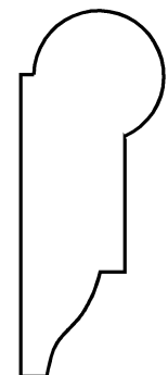
273 Picture Mould 11/16 x 1-3/4
