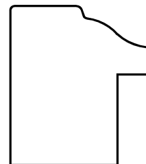
445 Back Band 1-7/32 x 1-1/16 (11/16" Rabbet)
