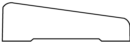
324 Casing 11/16 x 2-1/4
